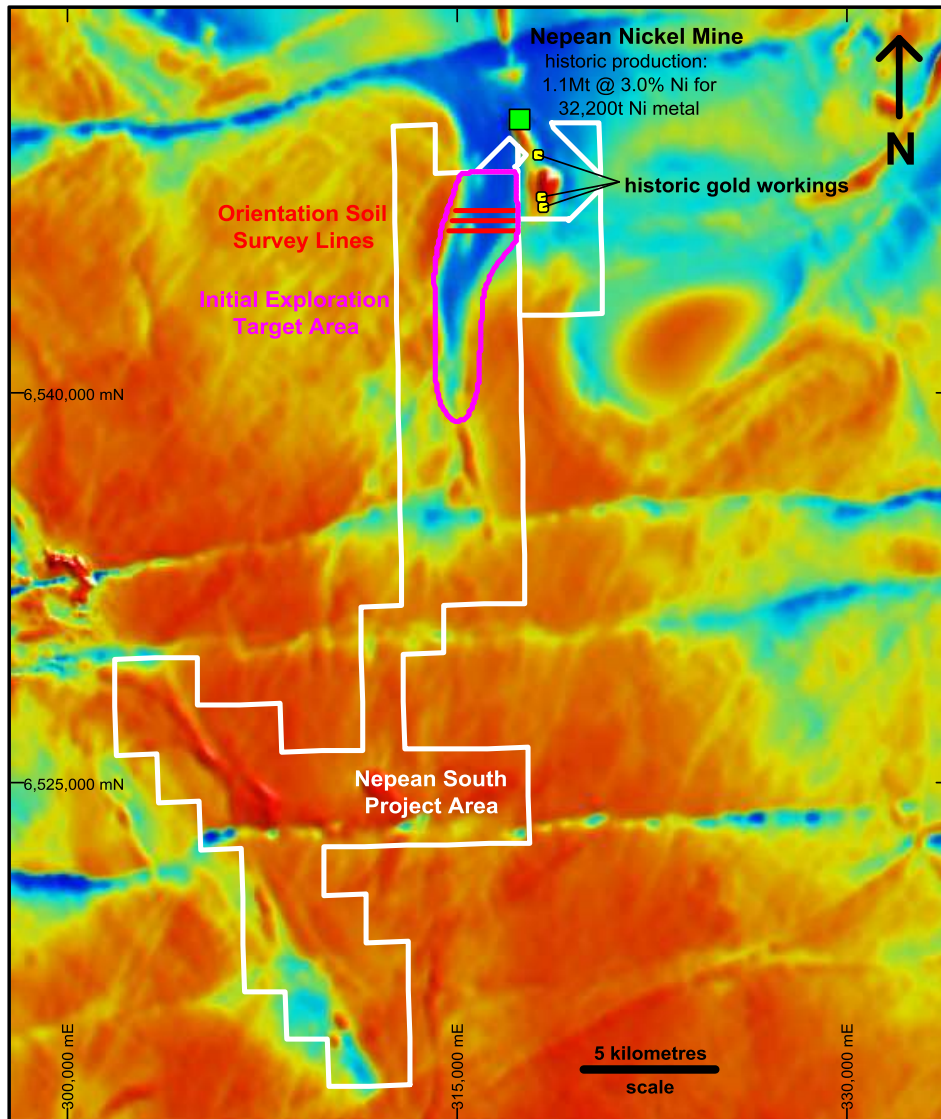
Figure 2: Nepean South, showing priority exploration target area and orientation soil survey lines on background aeromagnetic image.
